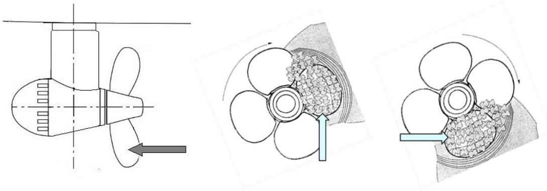
Figure 15. Location of the excitation on the blade.
