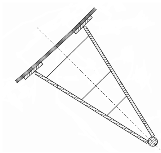
Figure 12. An example of an A-type bilge keel construction.
