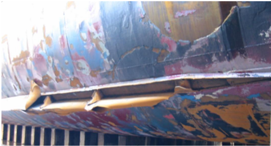
Figure 11. Damage caused by ice on the bilge keel of a ship. Please note that this is an example of damage caused by ice, not an example of good or bad design.
