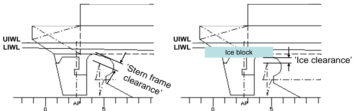
Figure 10. The clearance between the stern frame and the propeller (left) and the ice sheet and the propeller when the ship is at LIWL (right).
