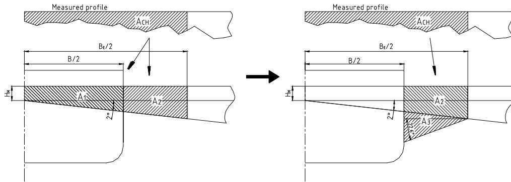
Figure 1. The geometry of a “real” brash ice channel profile and the corresponding profile of a rule channel before the ship’s passage, and the assumed behaviour of the ice during the passage. The relations between the cross-sectional areas are: A_{CH} = A_1 + A_2 = A_2 + A_3 .
