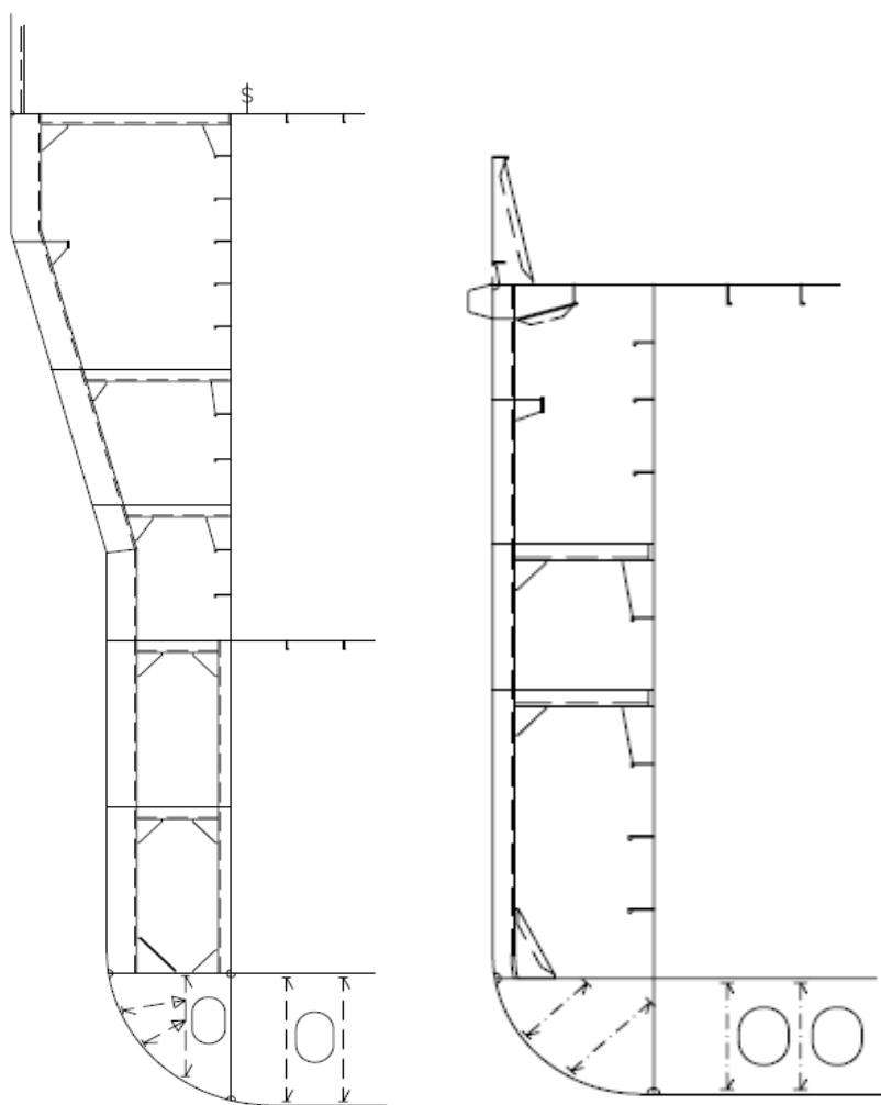
Figure 3a. Examples of frame connections.
