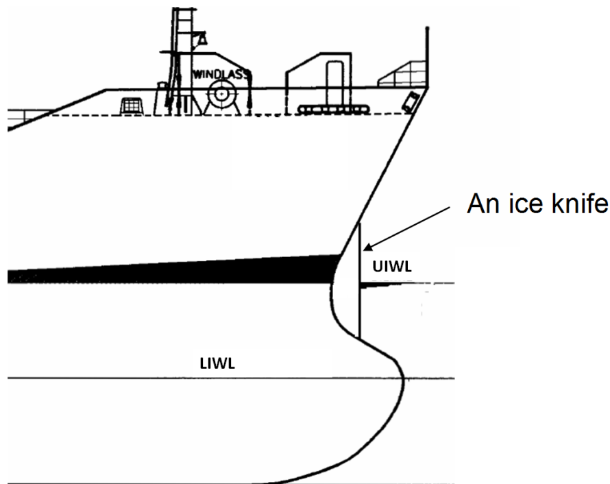
Figure 9. An ice knife is fitted on some ships.
